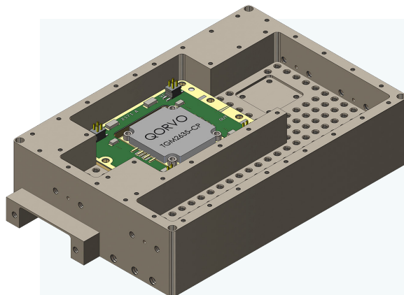
4. X-MWblock Drop-In in Integrated Microwave Assembly
