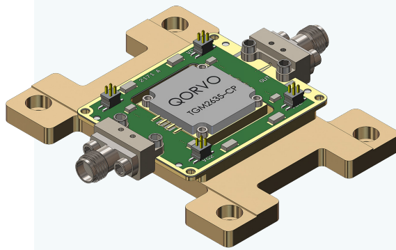
2. X-MWblock Drop-In on Copper Base and Heatspreader
