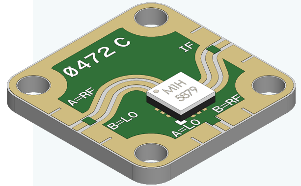
1. Drop-In X-MWblock
