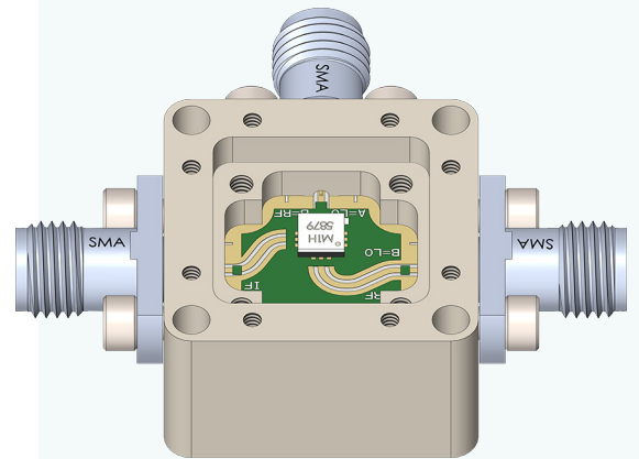
3. Drop-In in Connectorized Module
