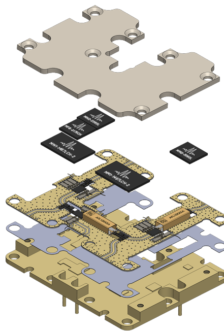
Marki Wire Bondable Die Mixers, Multipliers, and Filters in Custom Miniaturized Drop-In Dual Converter
