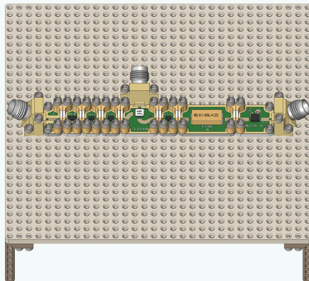
4. Drop-In in Prototype Plate Signal Chain
