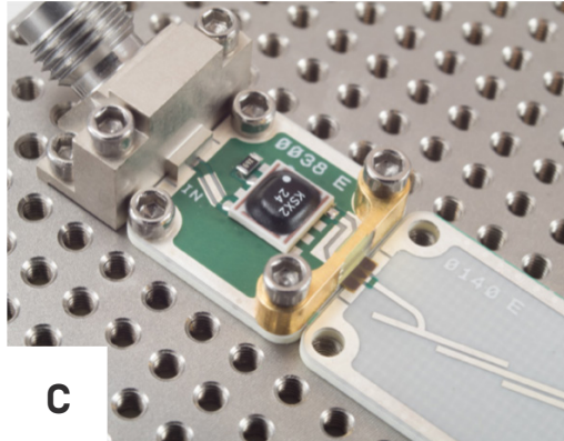
An X-MWanchor secures a jumper across the 5 mil air gap.
