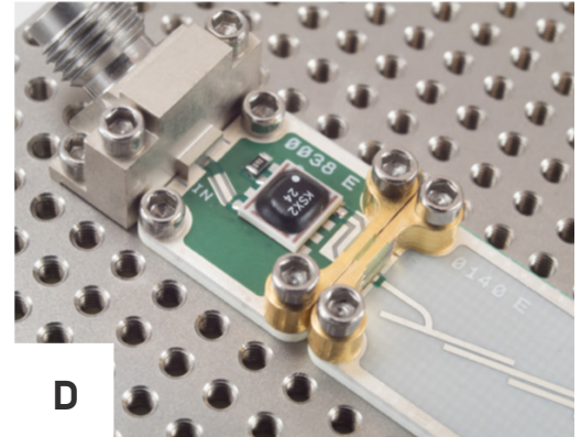
Each side of the GSG jumper is secured by an anchor.
